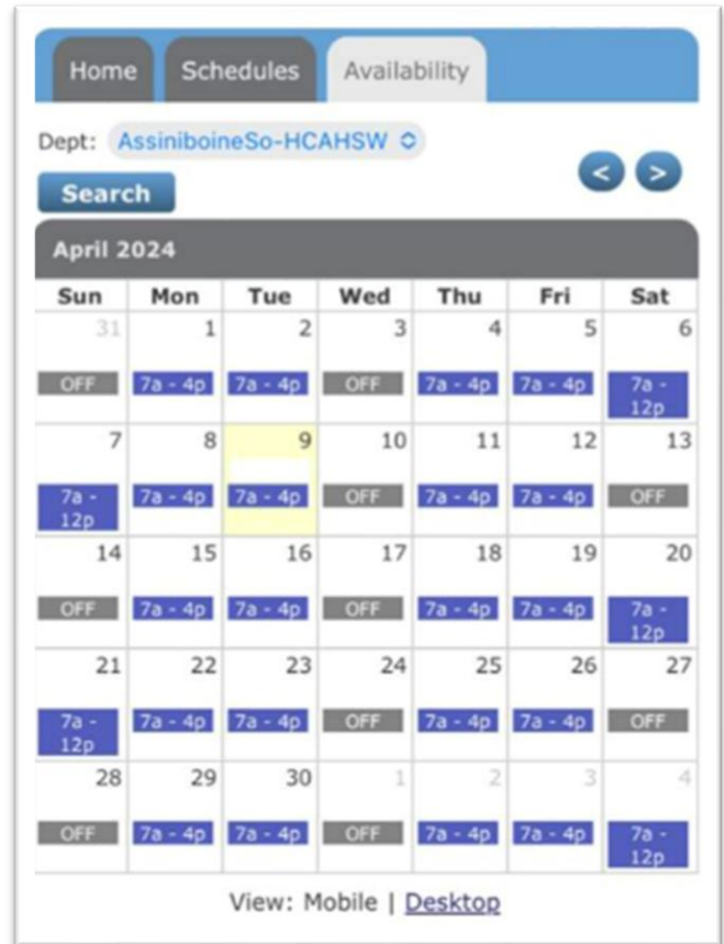
Figure 3 Availability Tab
